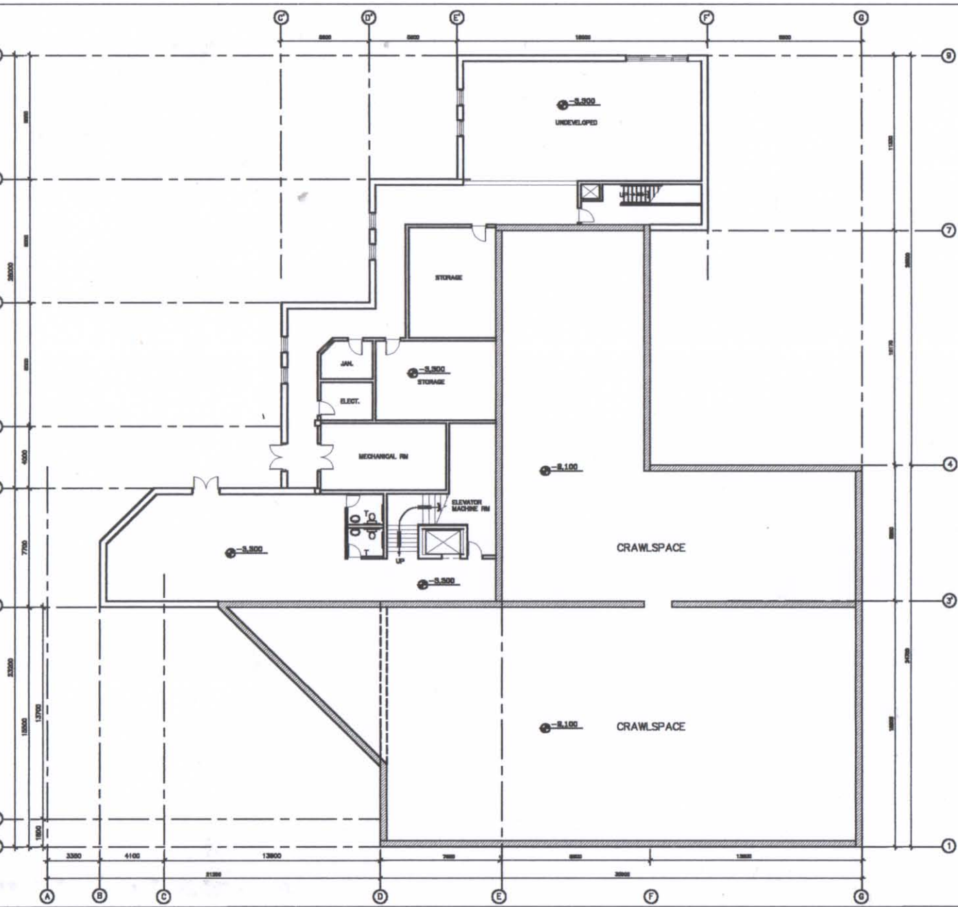
1 A-1 BASEMENT F 1:100
